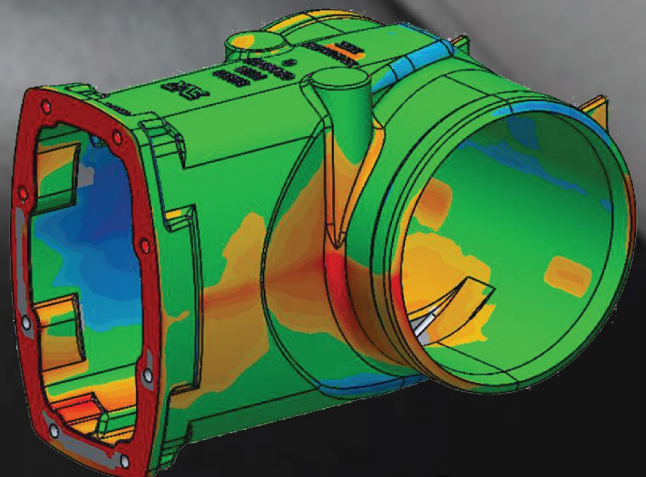
Advance Scanning Reports for Castings and Patterns
